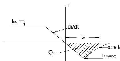
REVERSE RECOVERY CHARACTERIST
