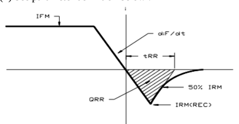
REVERSE RECOVERY CHARACTERISTIC
