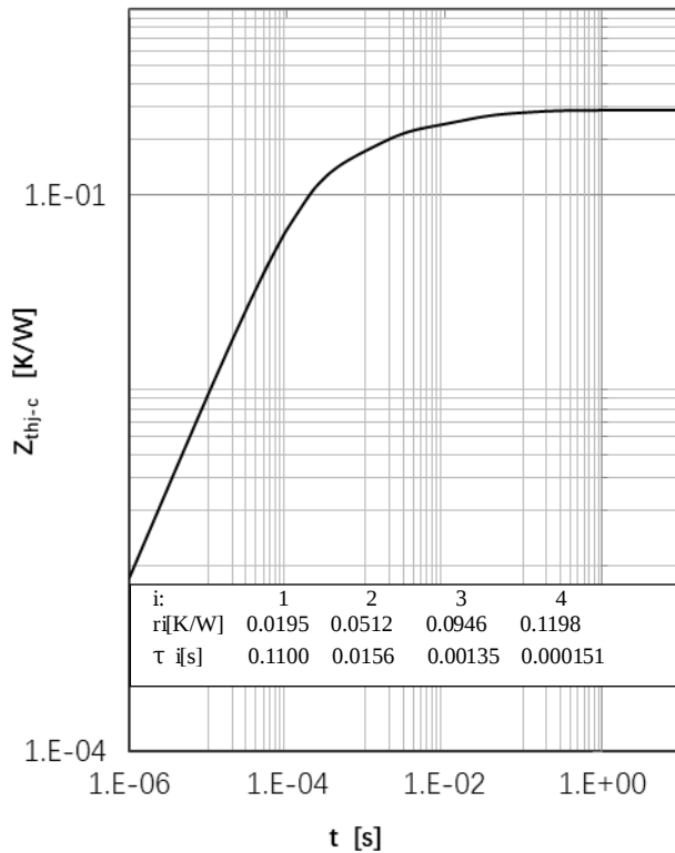
Fig 13. IGBT Transient Thermal Impedance
