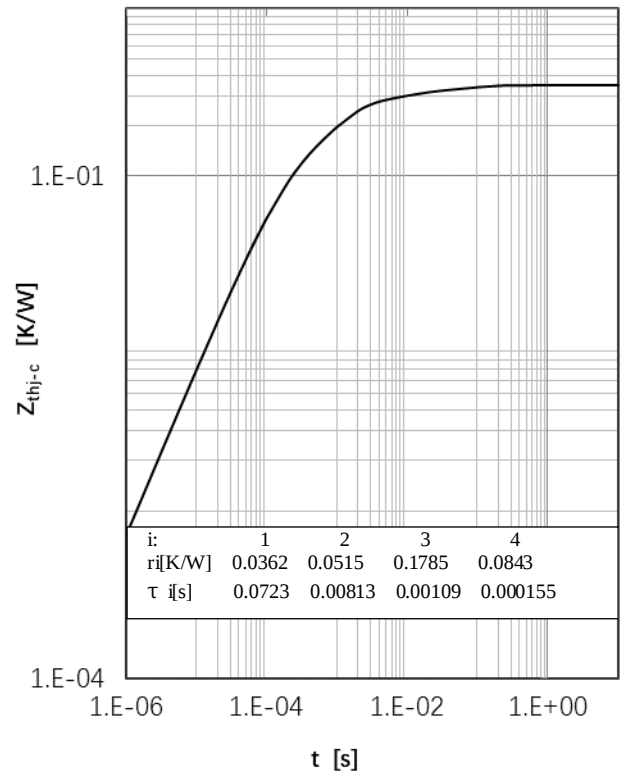
Fig 14. Diode Transient Thermal Impedance
