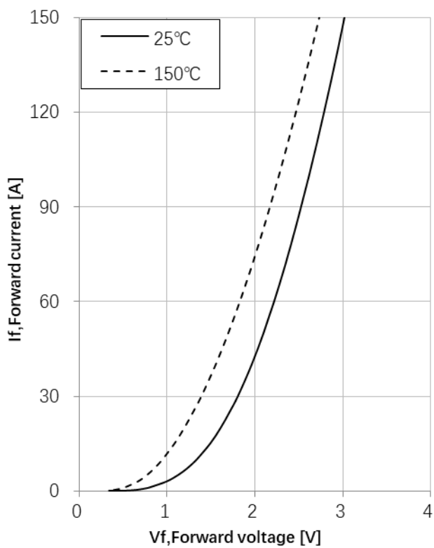
Fig15. Diode forward current as a function of forward voltage
