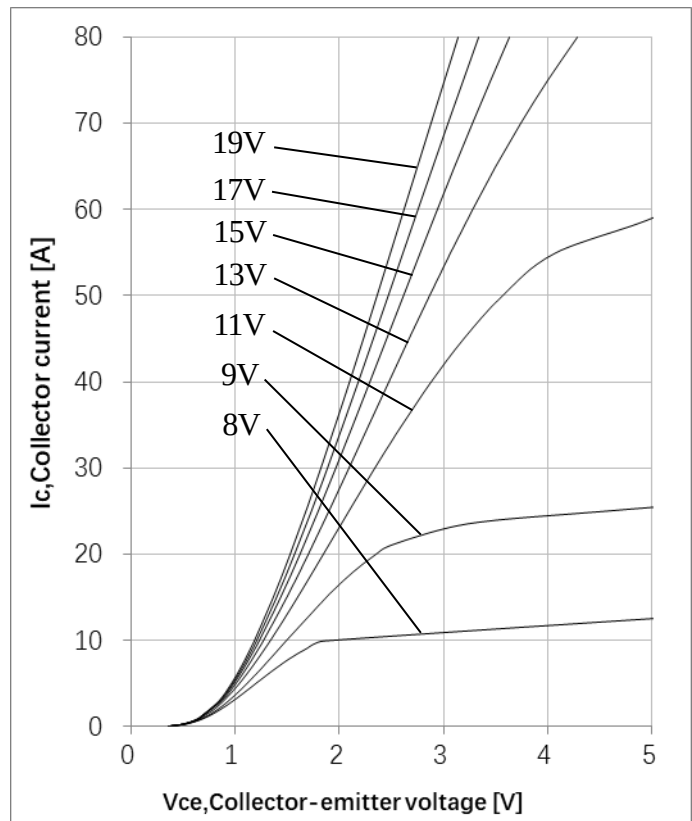
Fig4. Typical output characteristic ( T_j = 150^\circ\text{C} )
