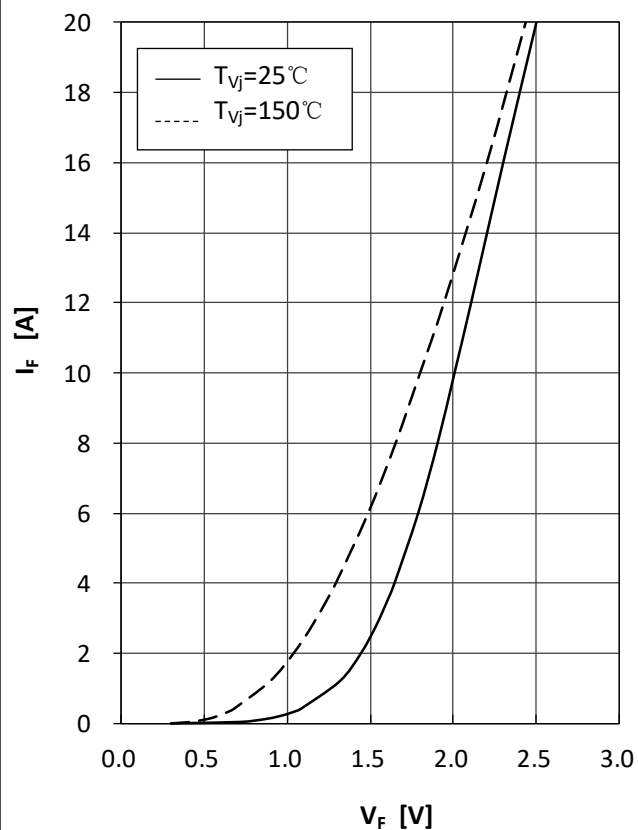
Fig13.Diode-brake-chopper Foward Characteristics
