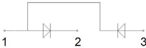
Circuit
