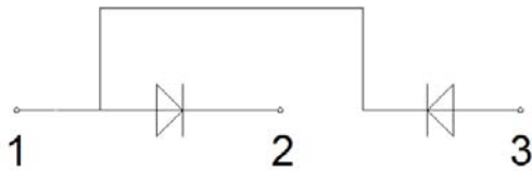
Circuit
