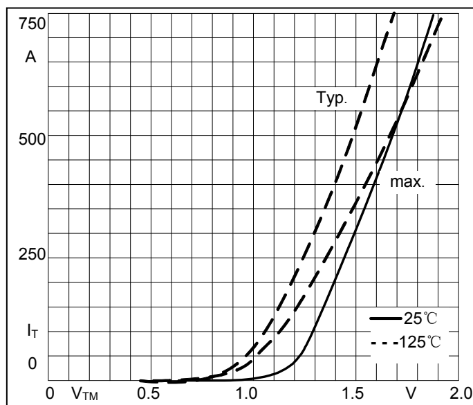
Fig5. Forward Characteristics
