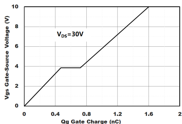
Figure4. Gate Charge
