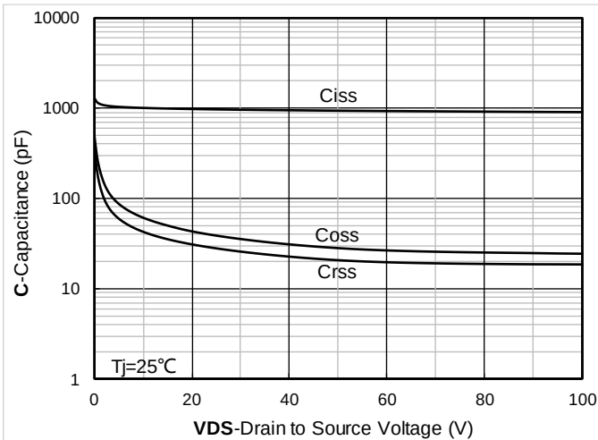
Figure 3. Capacitance Characteristics
