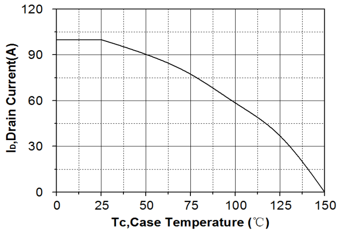
Figure7. Drain current
