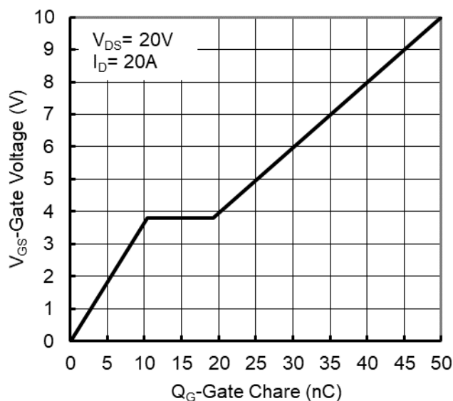
Figure 6. Gate Charge
