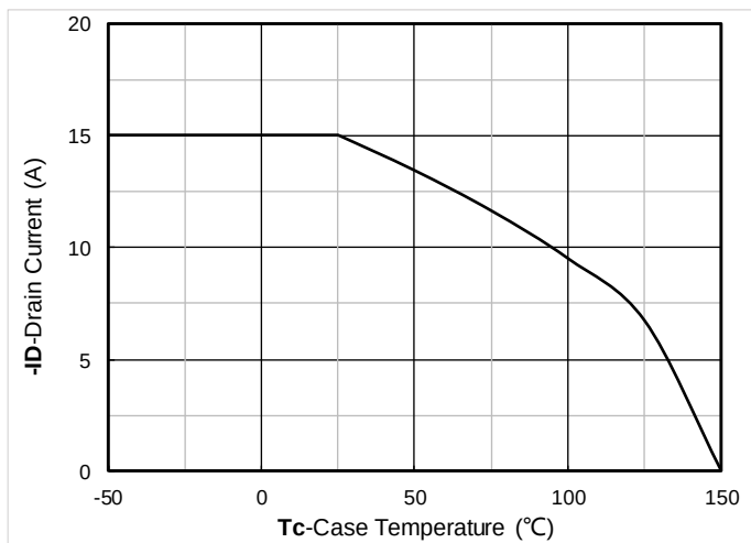
Figure7. Drain current
