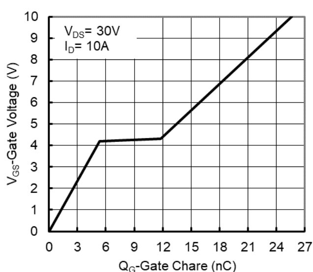
Figure 6. Gate Charge
