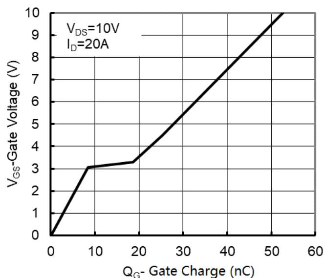
Figure 6. Gate Charge
