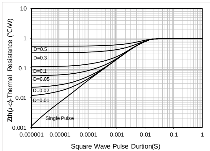
Figure 7. Maximum Transient Thermal Impedance
