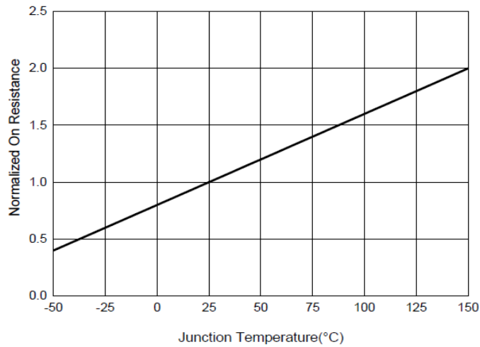
Figure 3. Normalized On-Resistance
