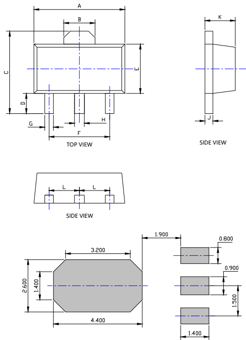
SUGGESTED SOLDER PAD LAYOUT
