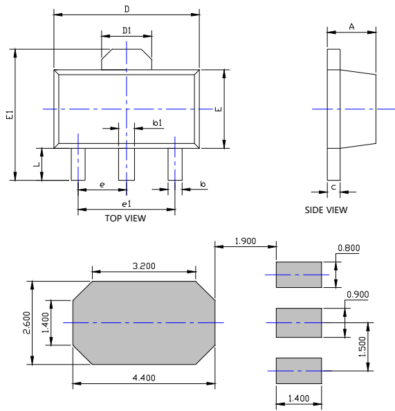
SUGGESTED SOLDER PAD LAYOUT
