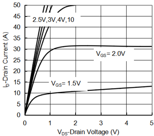
Figure1. Output Characteristics
