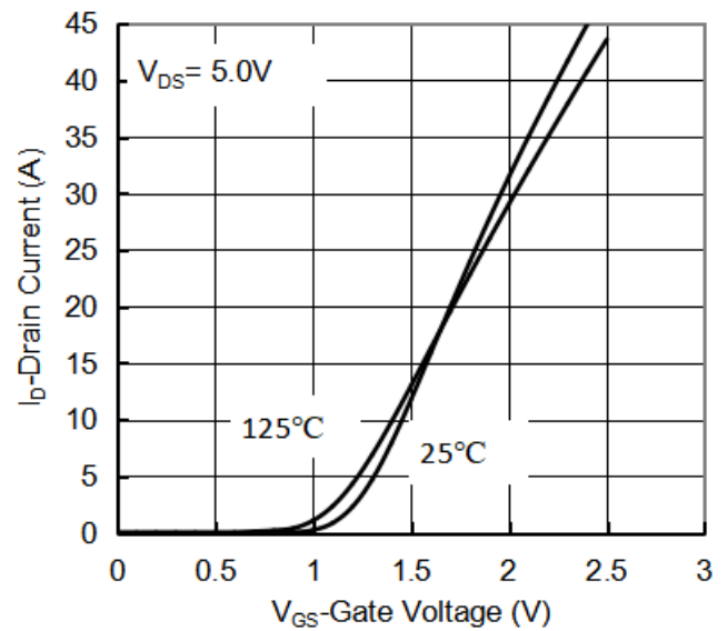
Figure2. Transfer Characteristics
