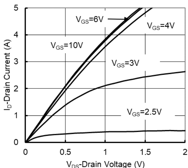
Figure1. Output Characteristics
