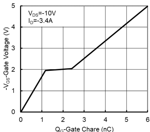
Figure6. Gate Charge
