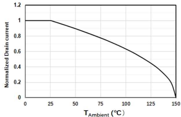
Figure8. Drain Current vs Ambient temperature
