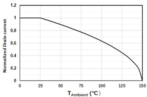
Figure8. Drain Current vs Ambient temperature
