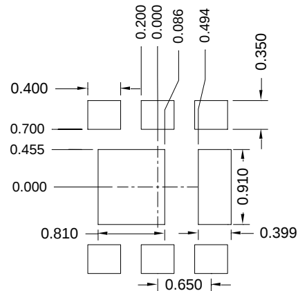
Suggested Solder Pad Layout Top View
