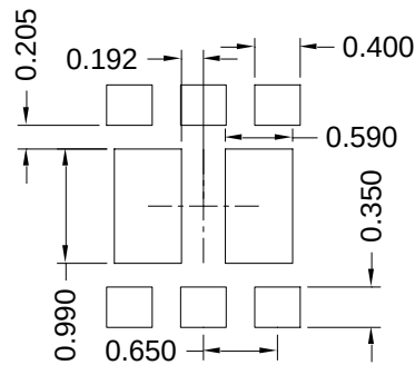
Suggested Solder Pad Layout Top View
