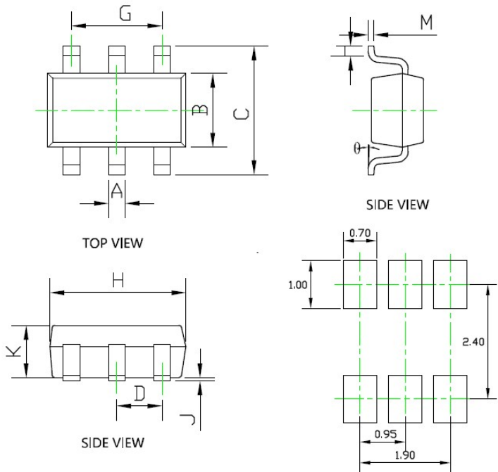
Suggested Solder Pad Layout
