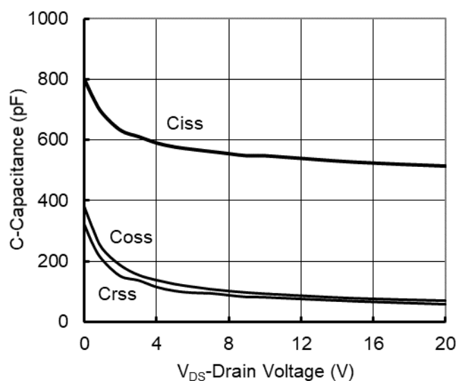
Figure5. Capacitance Characteristics
