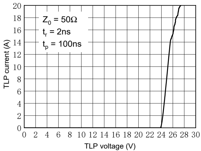
Fig.9 TLP Measurement
