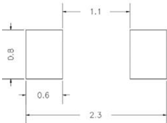
UNIT : mm SUGGESTED SOLDER PAD LAYOUT
