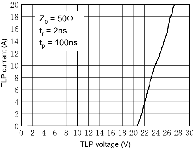
Fig.7 TLP Measurement
