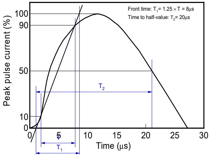
Fig.1 8/20 \mu s Waveform Per IEC6100-4-5
