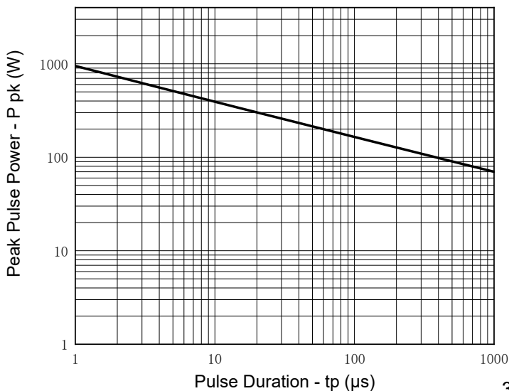
Fig.4 Non-Repetitive Peak Pulse Power vs Pulse
