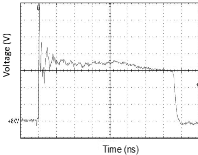
Fig.7 ESD clamping
