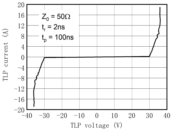
Fig.5 TLP Measurement
