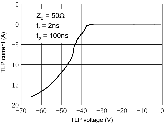
Fig.7 TLP Measurement
