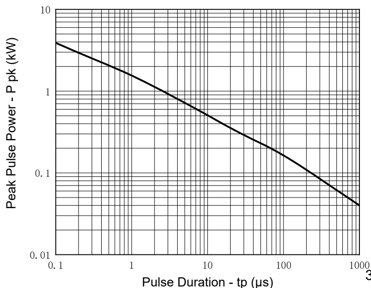
Fig.4 Non-Repetitive Peak Pulse Power vs Pulse Time
