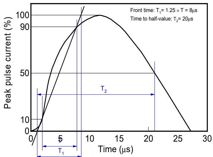
Fig.1 8/20us Waveform Per IEC6100-4-5
