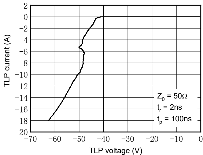
Fig.7 TLP Measurement
