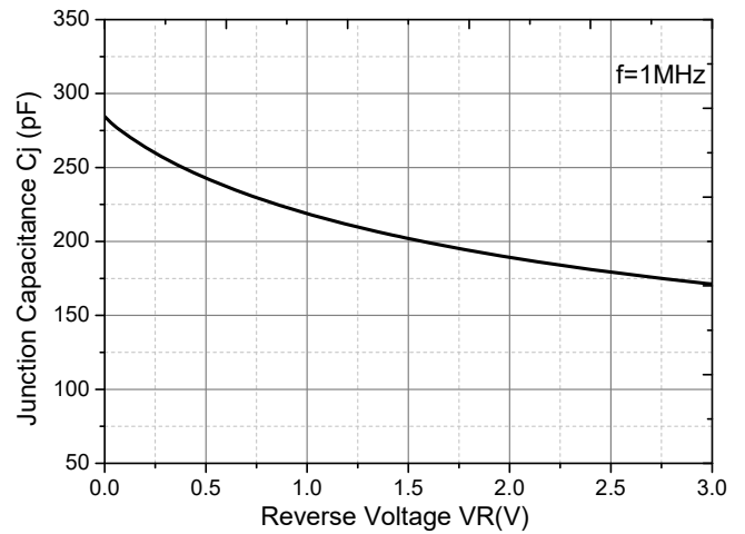
Figure 2. Capacitance Characteristics
