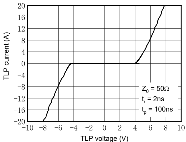
Fig. 9 TLP Measurement
