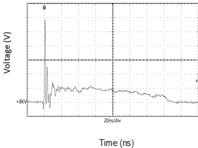
Fig.7 ESD clamping
