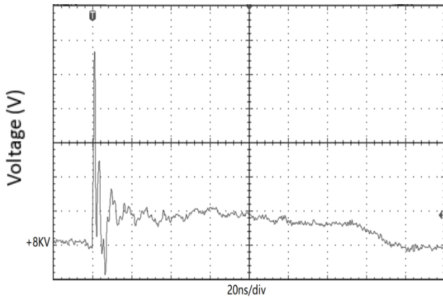
Fig.7 ESD clamping
