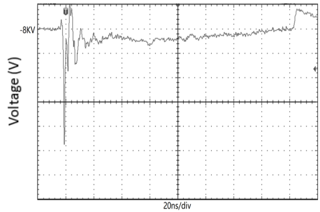
Fig.8 ESD clamping t
