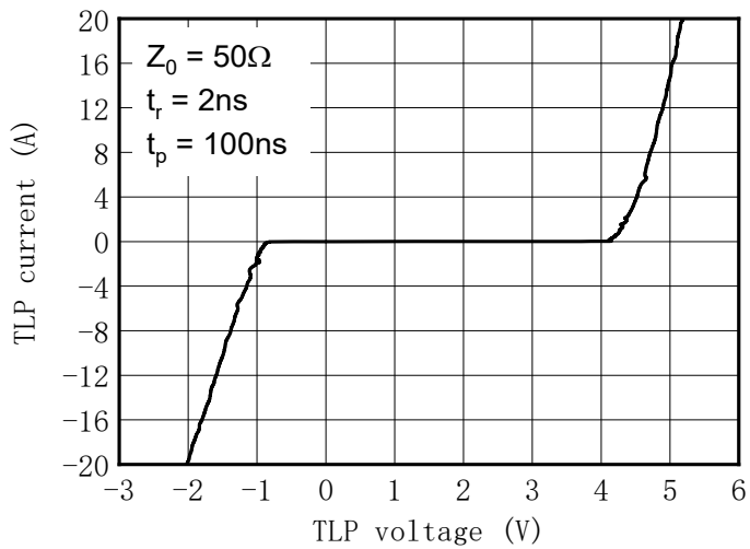
Fig.9 TLP Measurment
