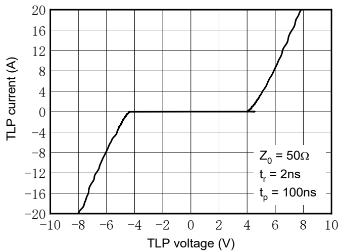
Fig. 9 TLP Measurment
