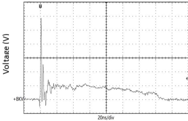
Fig.7 ESD clamping
