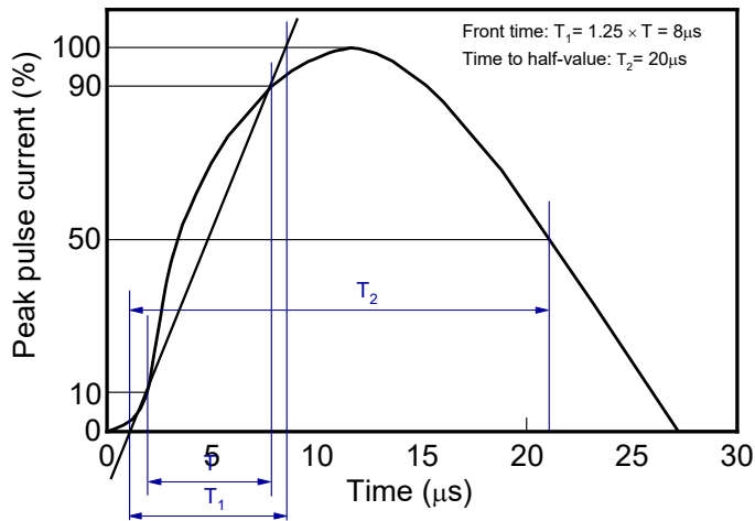
Fig.1 8/20 \mu s waveform per IEC61000-4-5
