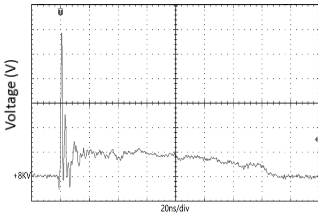
Fig.7 ESD clamping
