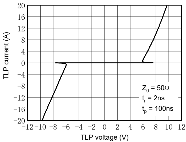
Fig. 9 TLP Measurment
