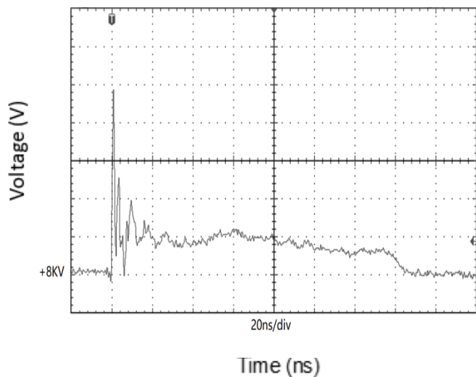
Fig.7 ESD clamping
