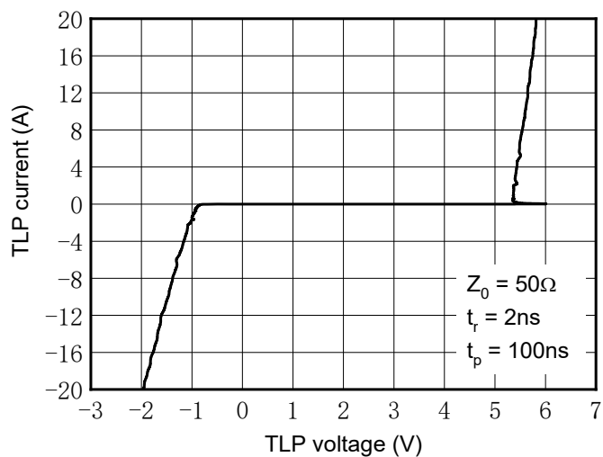
Fig. 9 TLP Measurment
