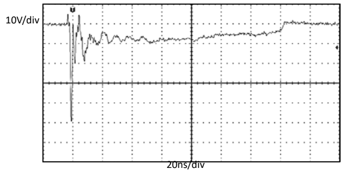
Fig.8 ESD clamping (-8kV contact discharge per IEC61000-4-2)
