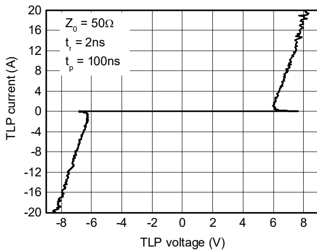
TLP Measurement
