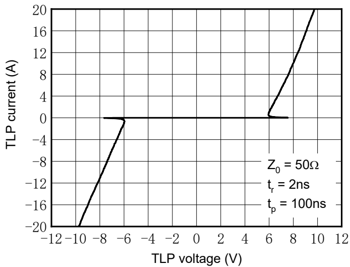
Fig.9 TLP Measurment
