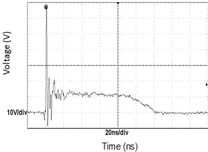
Fig.7 ESD clamping
