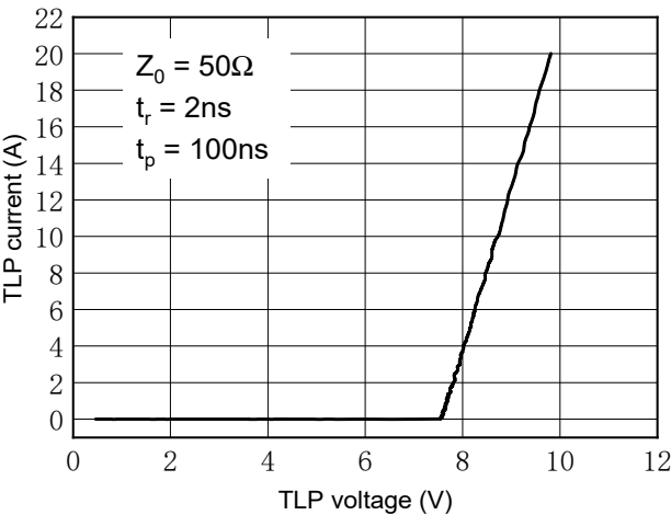
Fig.9 TLP Measurement
