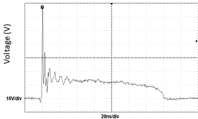
Fig.7 ESD clamping
