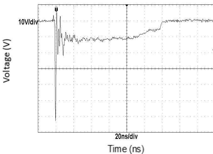
Fig.8 ESD clamping
