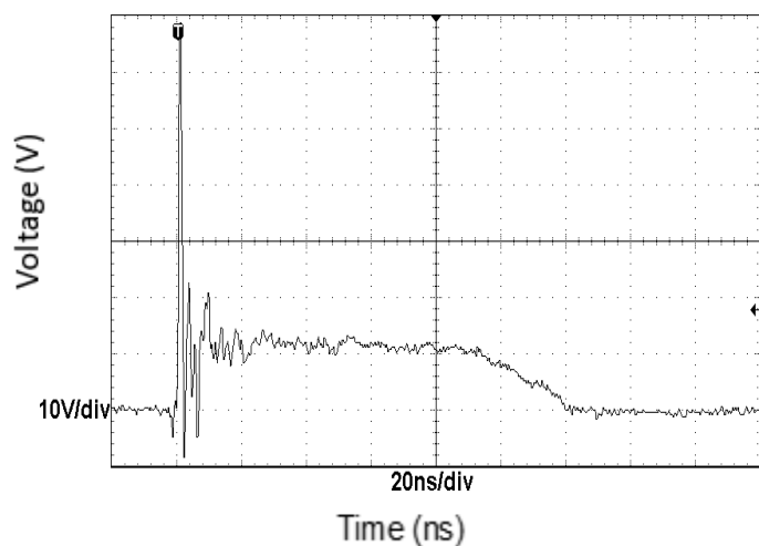
Fig.7 ESD clamping
