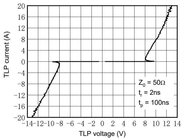
Fig.9 TLP Measurement
