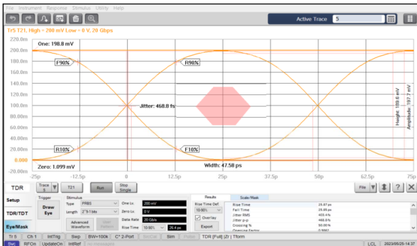
Fig 3(B) Eye pattern
