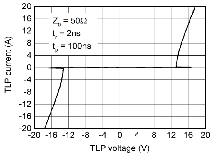
Fig.9 TLP Measurement
