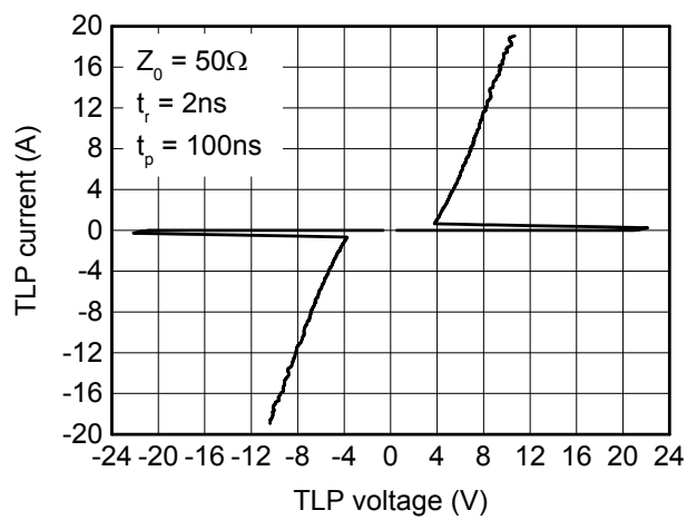
TLP Measurement
